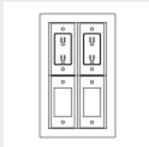
2 Duplexes 2 Data/Phone Audio/Video Faceplate
